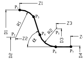
Figure 9 Non-tangent conjunction in P_3 point
