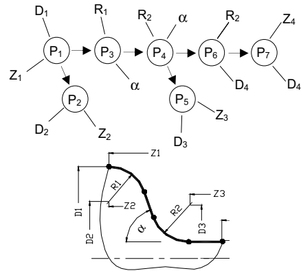
Figure 8 Parameterization scheme of half-open stair
