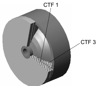
Figure 20 Implementation of CTF for typical part “Nakonechnik”
