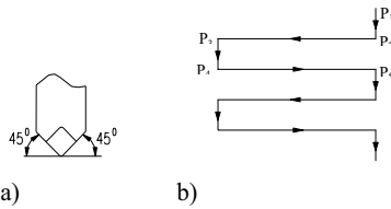
Figure 18 5 Point non-cycled rule of tool movement
