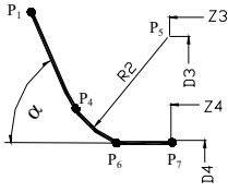
Figure 10 Non-tangent conjunction in P4 P6 points
