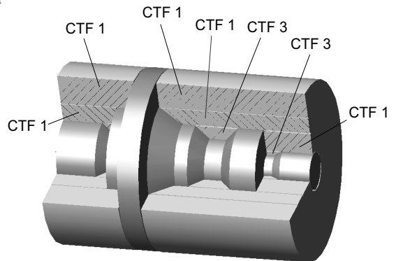
Figure 19 Implementation of CTF for typical part “Perehodnik”
