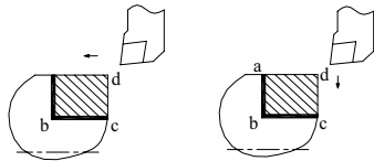
Figure 5 Consideration of base surfaces
