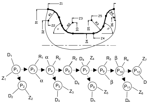
Figure 13 Parameterization scheme of STCL
