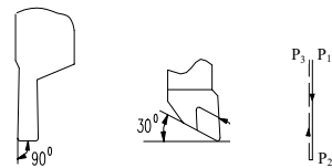
Figure 17 Tool set for machining of STCL
