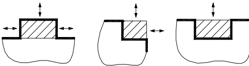
Figure 1 General types of manufacturing stocks
