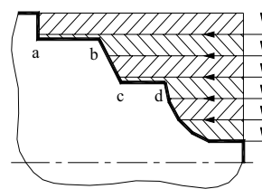
Figure 3 Stock distribution according to the depth of the cut
